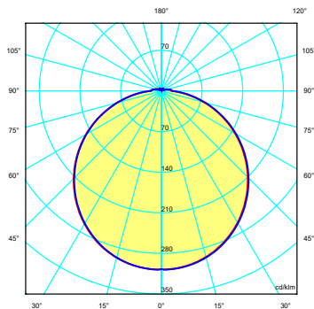
Beam angle 120°
